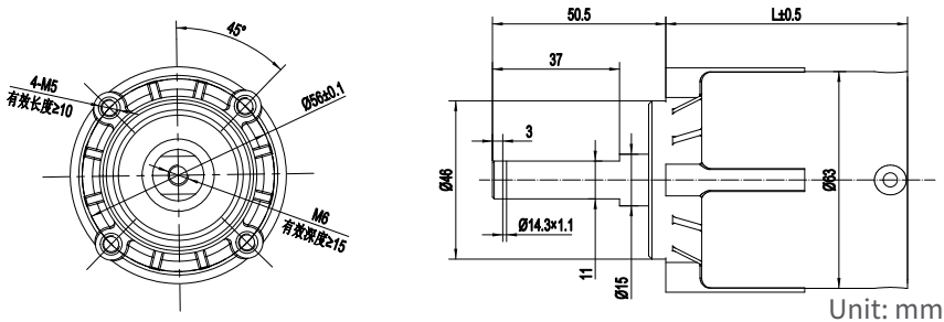
外型图/ Mechanical Dimension
